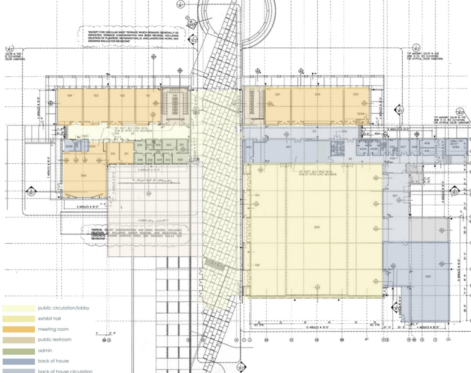
LEVEL ONE FLOOR PLAN | EXISTING
