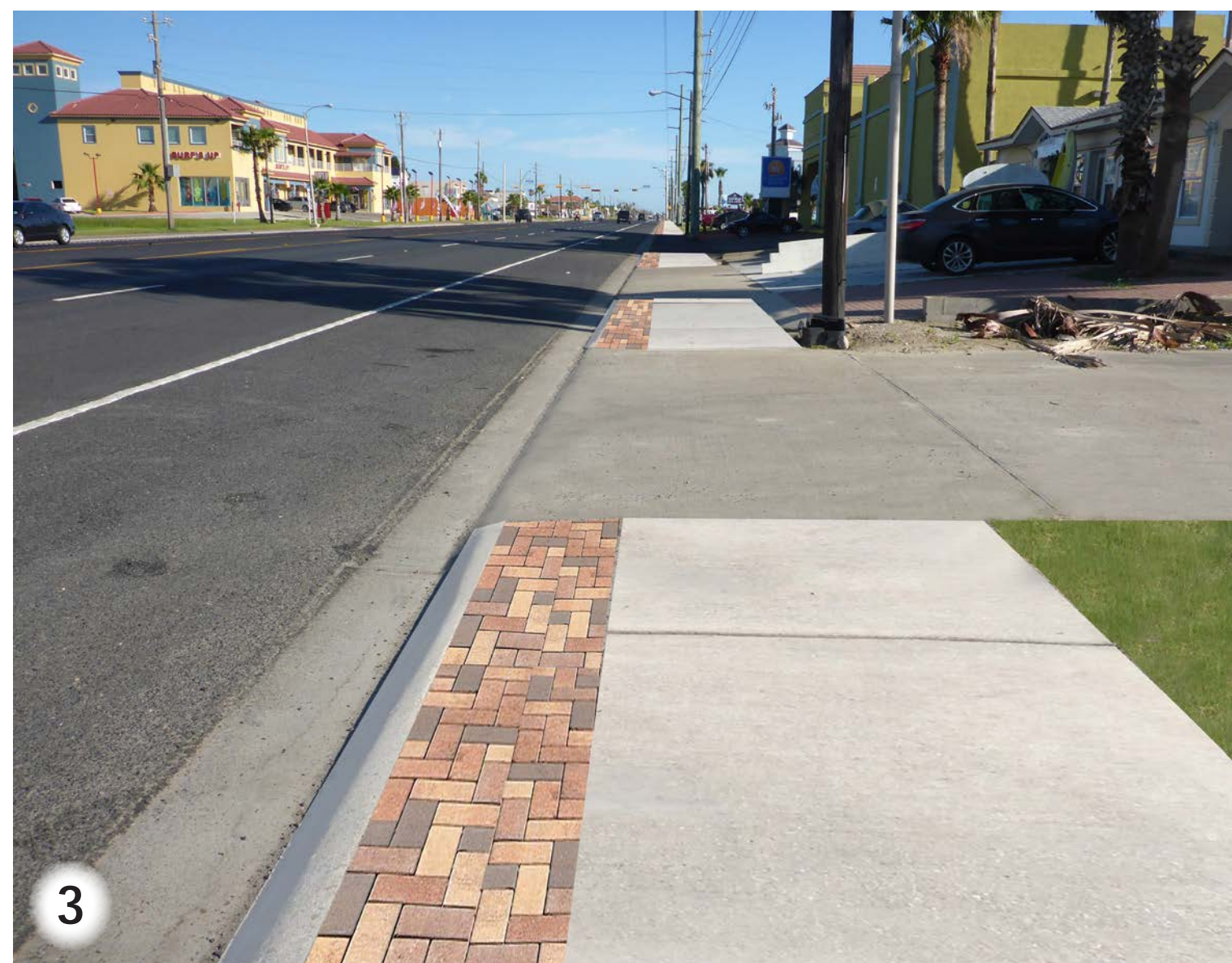
Proposed 6' Sidewalk w/ 2' Decorative Paving
